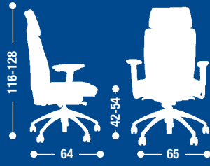
TK30 Poltrona ergonomica alta oscillante mov. 21. Hig ergonomic armchair w/tilting mov. 21.
