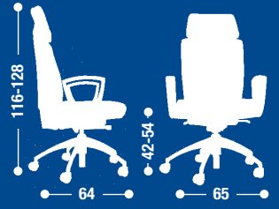
TK32 Poltrona ergonomica alta oscillante mov. 21. Hig ergonomic armchair w/tilting mov. 21.
